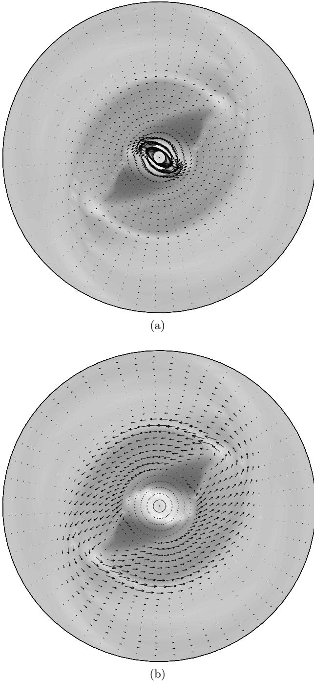
Fig. 4. Vectors of the horizontal magnetic field for the model with R_\alpha = 0.3 , R_\omega = 36 , f_\alpha = f_\eta = 0 . The circumscribing circle has radius 8 kpc. Shades of grey show gas density, with lighter shades corresponding to higher values. The magnetic field vectors have been rescaled by \mathbf{B} \rightarrow \mathbf{B}/B^n with n = 0.3 , to improve the visibility of the field vectors in regions with small B . Panel a) shows the field vectors over the entire computational domain, whereas in b) the inner region has been omitted, in order to show the structure in the outer regions of the disc.
