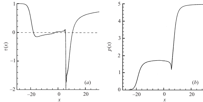
FIGURE 5. Calculations of (a) skin friction and (b) pressure distribution for \alpha = 5 ; solid line – method A (mesh 1001 \times 201 ); dotted line – method B (mesh 1400 \times 71 ).
