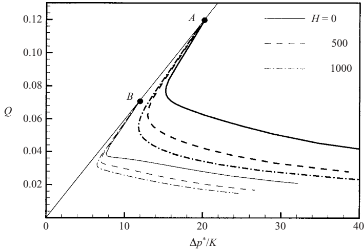
FIGURE 10. Volume flux, Q , as a function of pressure drop, \Delta p = p_{\text{up}} - p_{\text{down}} , for constant upstream transmural pressure. The different line thickness denotes two different upstream transmural pressures: P_{\text{tm}(\text{up})} = 0 (thick) and -2.5 (thin). The points at which the axisymmetric state becomes unstable to non-axisymmetric perturbations is indicated by A ( P_{\text{tm}(\text{up})} = 0 ) and B ( P_{\text{tm}(\text{up})} = -2.5 ).
