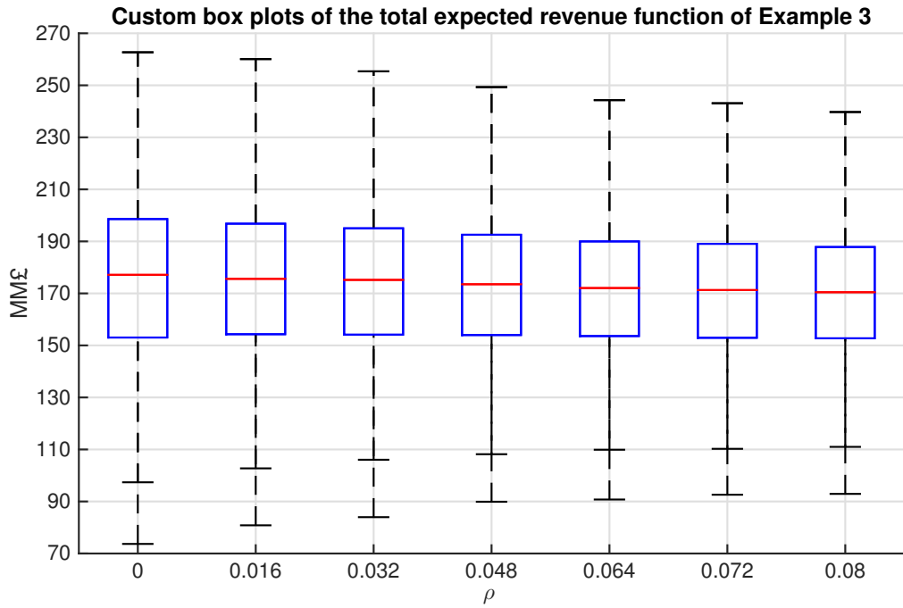
Figure 6.8: Custom box plots of the total revenue function of Example 3. The two lower whiskers below each box indicate the risk measures CVaR_{95\%} and CVaR_{99\%} . The red line is the median, the edges (top and bottom) of the box are the 25th and 75th percentiles, the upper whisker is the highest datum that is not an outlier, i.e. it is still within 1.5IQR (interquartile) of the upper quartile.
