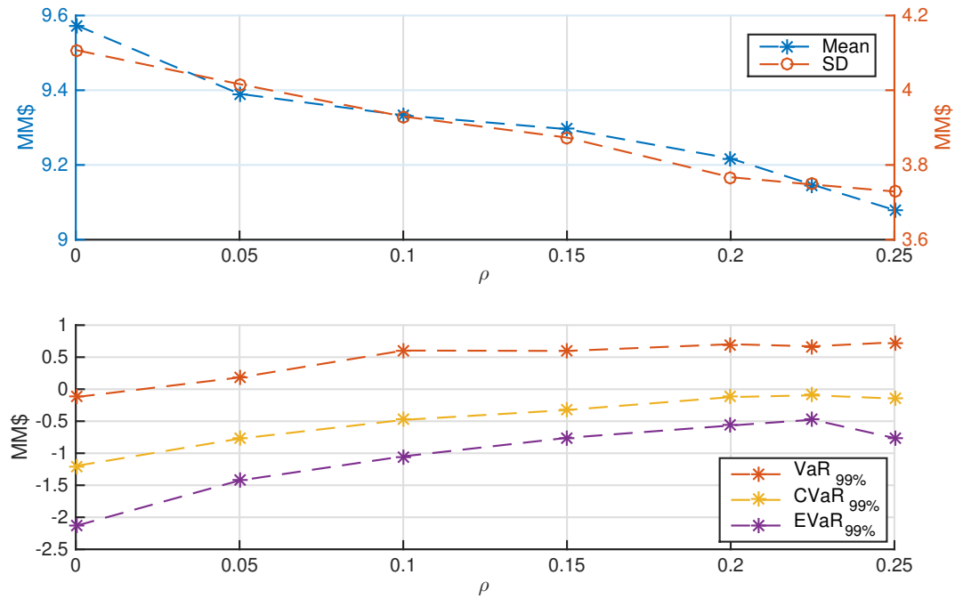
Figure 6.5: For the total revenue function of Example 2, its mean, standard deviation (SD) and risk measures VaR, CVaR and EVaR all at the 99% confidence level, as a function of the degree of risk-sensitivity \rho . In this example the greater the risk measures the smaller the risk faced by the plant operator. The results are based on 2000 sample paths.
