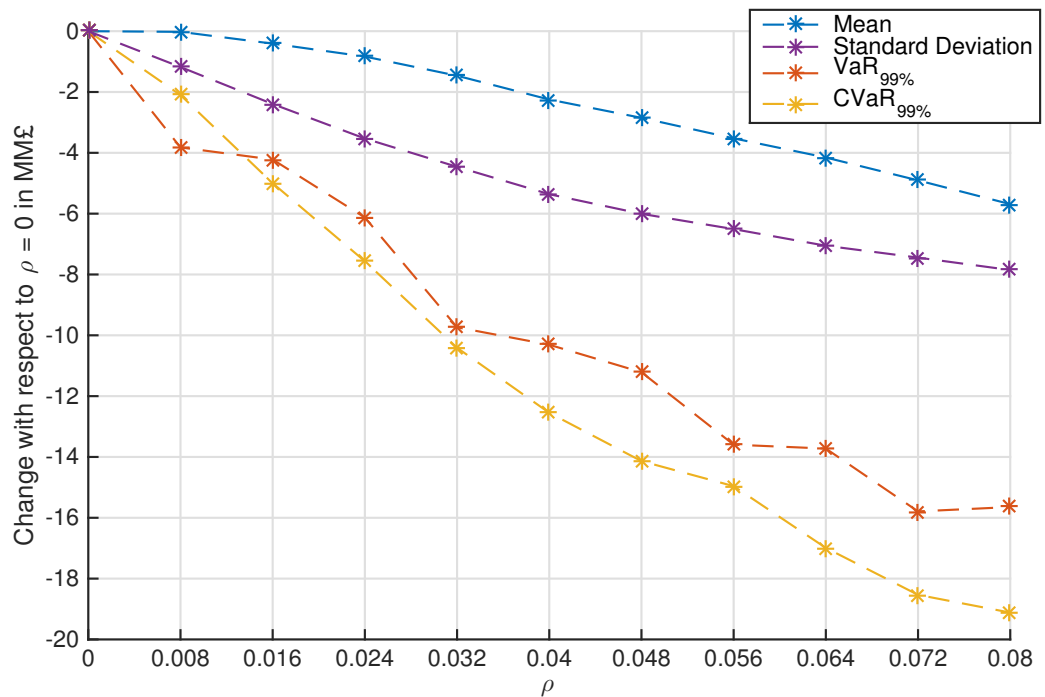
Figure 6.9: Change with respect to the risk-neutral case \rho = 0 in the expected total revenue (mean), and risk measures VaR_{99\%} and CVaR_{99\%} as \rho increases. A negative value means that the corresponding index has decreased.
