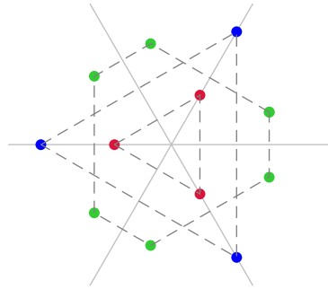
Figure 1: A configuration with triangular ( D_3 ) symmetry, consisting of 12 points forming 3 orbits: two equilateral triangles and one semiregular hexagon. The theorem guarantees the existence of a central configuration of this form, where the relative sizes will depend on the relative masses of each of the 3 orbits.
