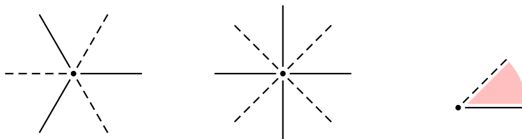
Figure 3: The connected components of the fixed point sets for actions of D_3 and D_4 , with the orbit space \mathbb{R}^2/D_n with its 4 strata represented on the right.
