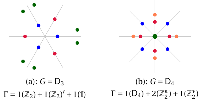
Figure 2: D_3 and D_4 symmetric configurations in the plane, taking connected components into account for D_3 . For D_4 , \kappa represents the reflection in the horizontal axis, and \nu in a diagonal axis.
