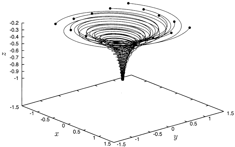
Fig. 9. The streamlines for a non-zero F solution obtained at \mu = 1/2 and Re = 2 . This pattern of streamlines is repeated (but inverted) in the upper half of the domain since the solution is symmetric about the midplane. The streamlines shown originate from a square of starting points (as illustrated by the circular points) in the plane z = -0.2 .
