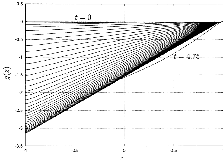
Fig. 19. g(z) profiles, \mu = 7.5 , \gamma = 0 , Re = 40 , \delta = 1 .
