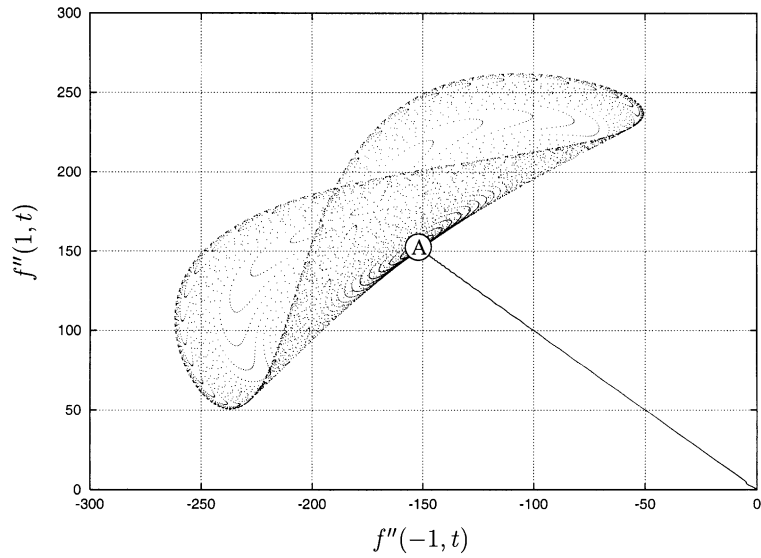
Fig. 8. An evolution of the unsteady boundary-value problem to a limit cycle solution (arising through a Hopf bifurcation) at \mu=0 , Re=10 . Point A denotes the location of the steady solution in this phase plane, corresponding to the axisymmetric “bifurcation to swirl” state as described by Goldshtik and Javorsky (1989).
