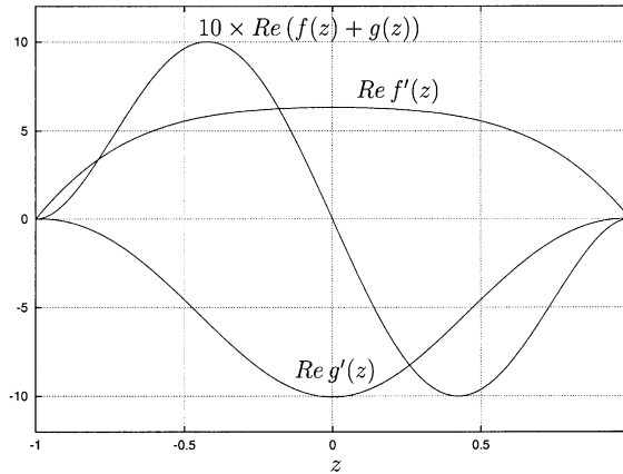
Fig. 2. The leading-order solution of the low-Reynolds non-axisymmetric state. Note that this is one of the non-trivial Re = 0 states shown in Fig. 1, the other state simply corresponds to an interchange of f and g .
