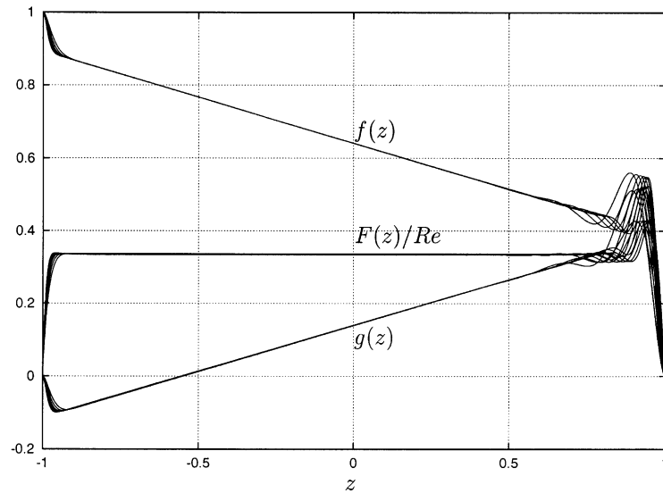
Fig. 14. Solution profiles for \mu = 1, \gamma = 0, Re = 50, 60, 70, 80, 90, 100 (larger values of Re exhibit larger solution gradients near boundaries).
