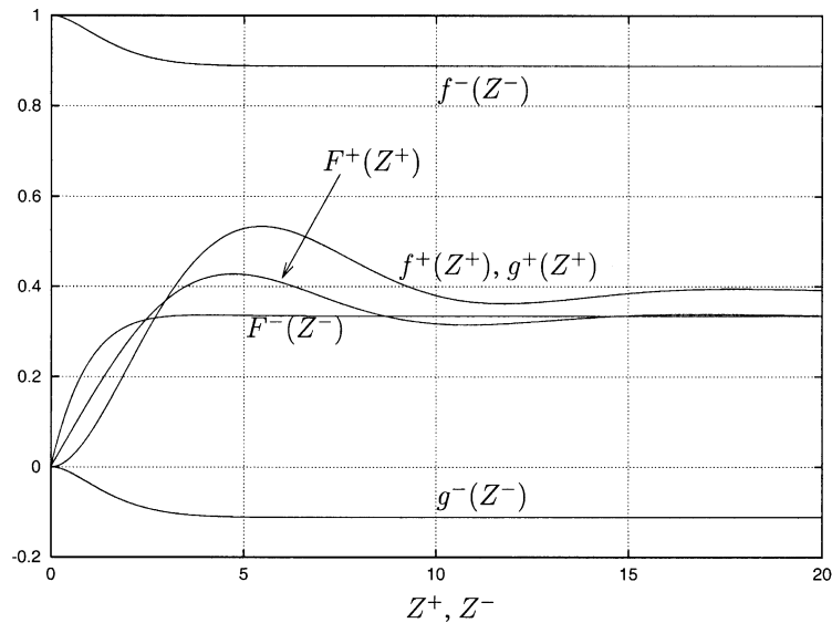
Fig. 15. Asymptotic solution profiles (near boundaries).
