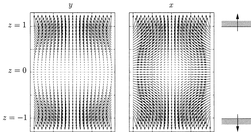
Fig. 7. The flow field in the x-z and y-z planes for a non-zero F solution obtained at \mu = 1/2 and Re = 2 . Note that the mass flux in the x -direction is three times that in the y -direction when \mu = 1/2 .
