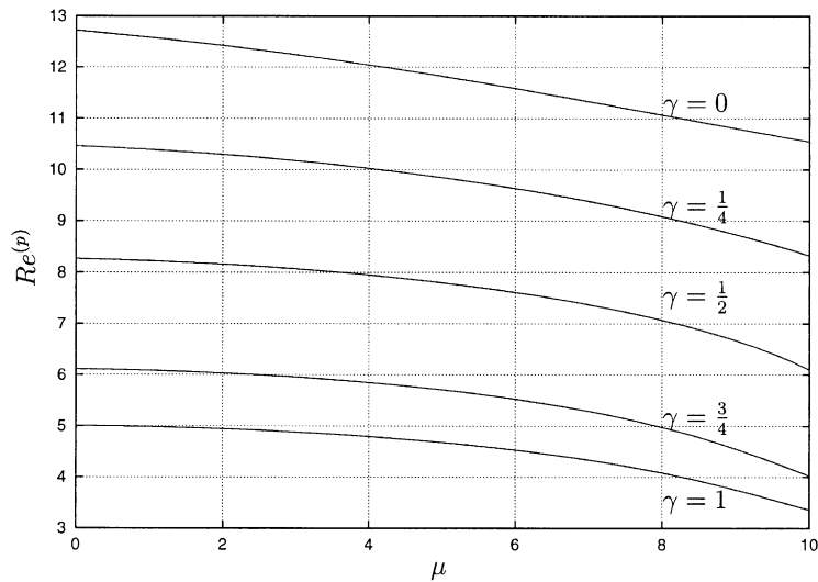
Fig. 11. Location of Hopf bifurcation from states with F \neq 0 in the case \delta = -1 .
