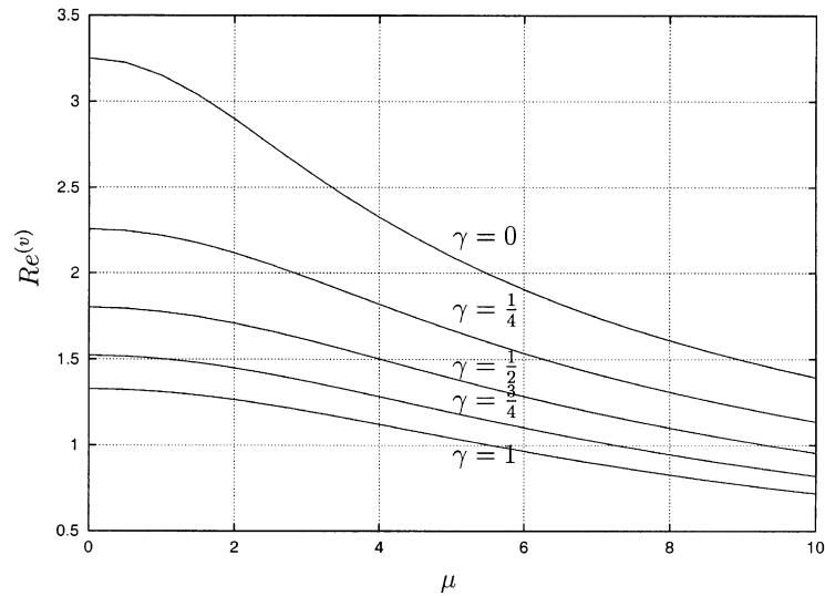
Fig. 10. Location of pitchfork bifurcation from states from F \equiv 0 to F \neq 0 in the case \delta = -1 .
