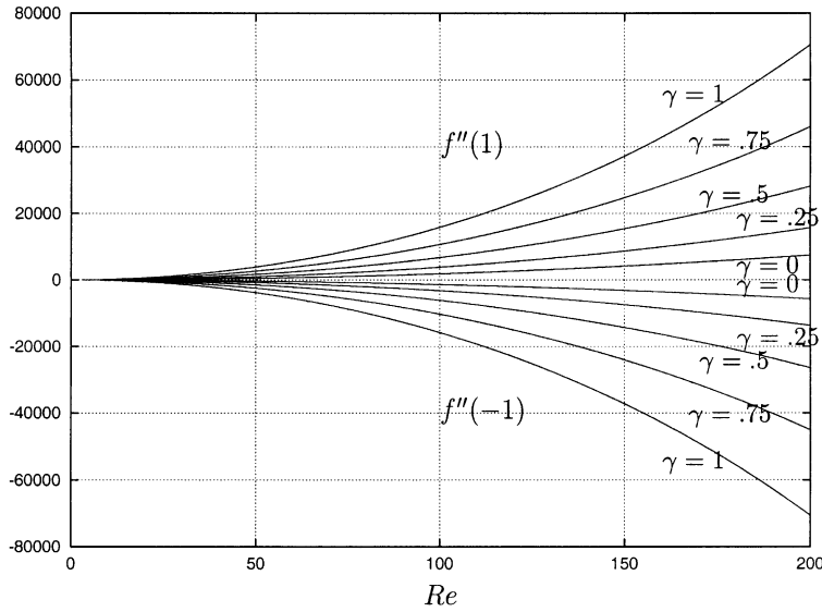
Fig. 12. Variation of f''(\pm 1) with Re at \gamma values as shown, \mu = 1 , \delta = -1 .
