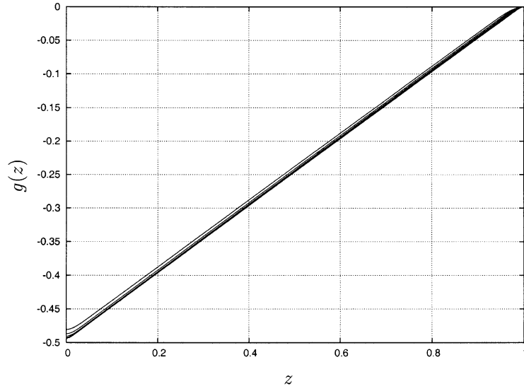
Fig. 5. g(z) profiles for f'''(-1) = 1000, 2000, 4000, 8000, 16000, 32,000 ( \mu = 1.960756, 1.973276, 1.980298, 1.984152, 1.986205, 1.987244 , respectively), on the solution branch of Fig. 3 with \gamma = 0, Re = 20, \delta = 0 .
