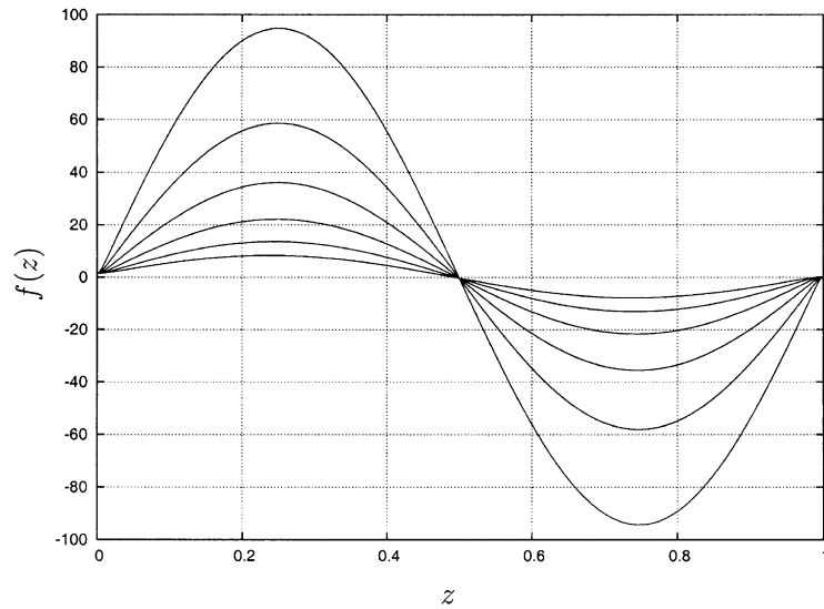
Fig. 4. f(z) profiles for f'''(-1) = 1000, 2000, 4000, 8000, 16,000, 32,000 ( \mu = 1.960756, 1.973276, 1.980298, 1.984152, 1.986205, 1.987244 , respectively), on the solution branch of Fig. 3 with \gamma = 0 , Re = 20 , \delta = 0 .
