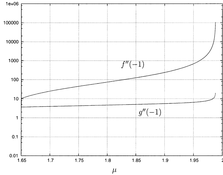
Fig. 3. Development of f''(\pm 1) and g''(\pm 1) for varying \mu with \gamma = 0 , Re = 20 , \delta = 0 . The calculations begin on the solution branch that may be continued to the low-Reynolds number limit.
