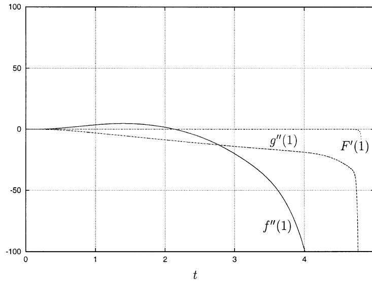
Fig. 17. Temporal development of f''(1) , g''(1) and F'(1) ; \mu = 7.5 , \gamma = 0 , Re = 40 , \delta = 1 .
