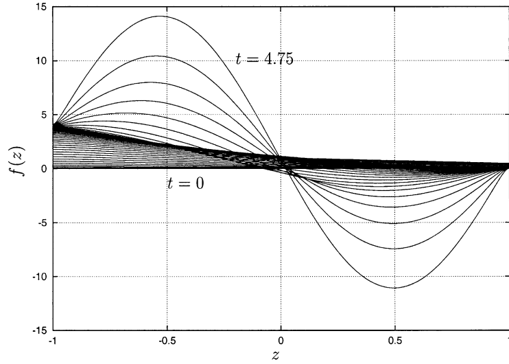
Fig. 18. f(z) profiles, \mu = 7.5 , \gamma = 0 , Re = 40 , \delta = 1 .
