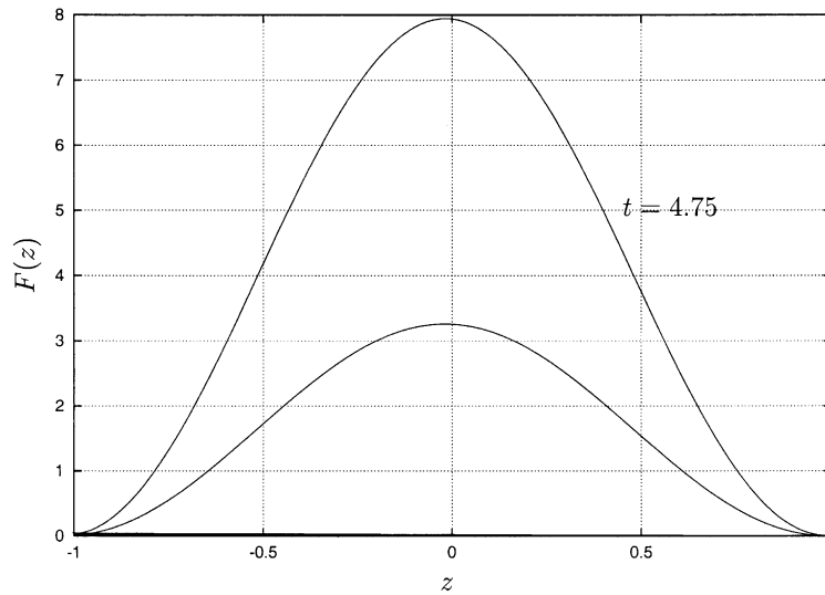
Fig. 20. F(z) profiles, \mu = 7.5 , \gamma = 0 , Re = 40 , \delta = 1 .
