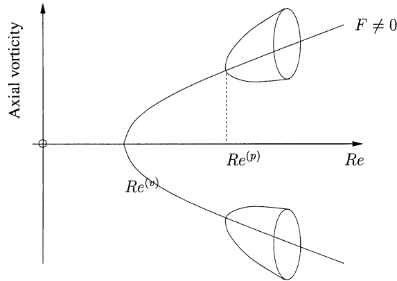
Fig. 6. The bifurcation diagram for the transition to states with non-zero F (equivalent to the generation of axial vorticity) for a fixed \mu . Here, Re^{(v)} denotes the pitchfork bifurcation to states of non-zero axial vorticity, whilst Re^{(p)} indicates the secondary instability via supercritical Hopf bifurcation.
