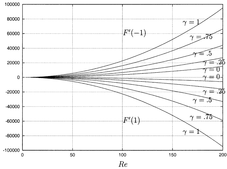
Fig. 13. Variation of F'(\pm 1) with Re at \gamma values as shown, \mu = 1, \delta = -1 .
