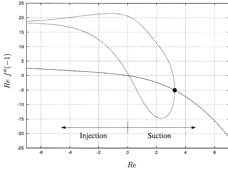
Fig. 1. The appearance of a non-axisymmetric injection state (shown as a dashed line) through a sub-critical pitchfork bifurcation in the suction regime and its continuation (through a singular solution in the low- Re limit) to the injection flow regime. Note that the two branches of the pitchfork correspond to an interchange of f and g .
