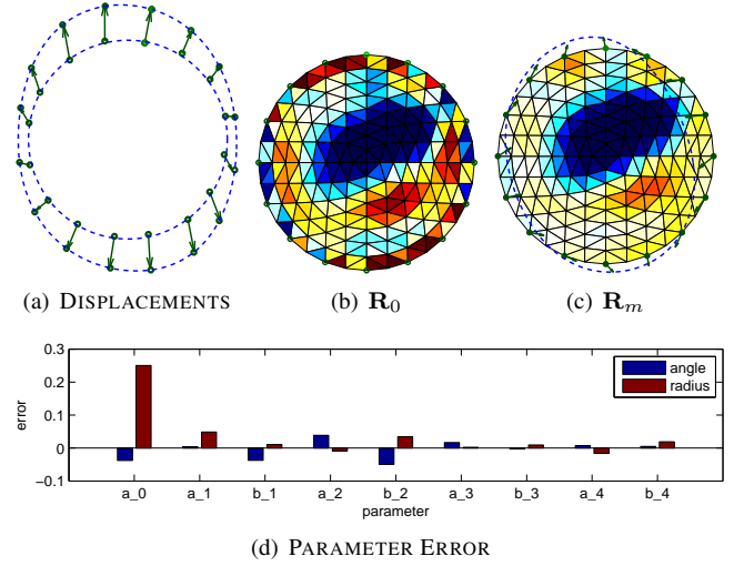
Fig. 12: Boundary reconstruction from electrode movement: 3-point compression with insulating target
