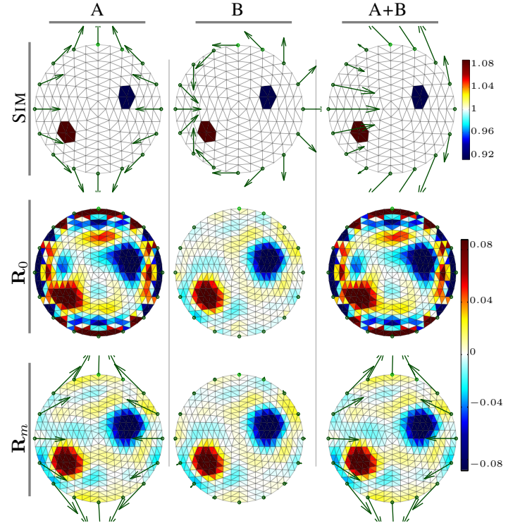
Fig. 8: Images reconstructed from three different movement patterns, illustrating that conformal distortion fields cannot be distinguished from conductivity changes. Green arrows indicate electrode movement ( 40\times exaggeration).
