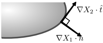
Fig. 6: Derivatives of the components of a conformal vector field at the boundary
