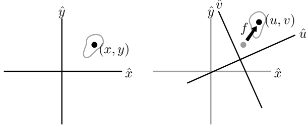
Fig. 1: A change of coordinate systems transforms the point (x, y) to the new coordinates (u, v) ; the old coordinates (x, y) relative to the original x -, y -axes are at the same location as the new coordinates relative to the new axes where in this case, a translation and rotation have been applied. The transformation need not lead to a rectilinear coordinate system.
