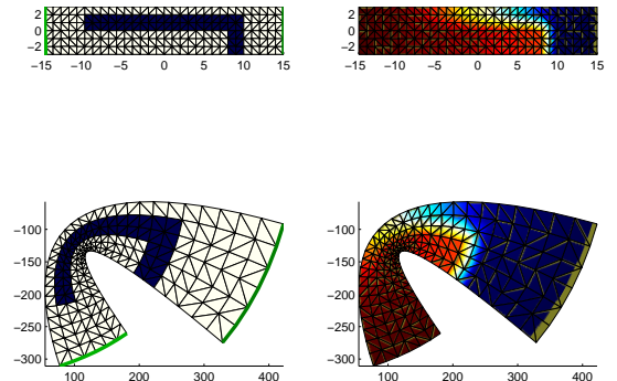
Fig. 5: A conformal mapping of a rectangular grid with the conformal map z \rightarrow \exp((z - 20 - i80)/100) \cdot (z + i20) \cdot (z - i10) , top – rectangular region with electrodes across the ends and L-shaped inhomogeneity, bottom – conformal deformation applied to FEM mesh prior to simulation, left – FEM mesh and inhomogeneity, right – simulated voltage distributions. Lines still intersect at 90^\circ after deformation. Voltages at individual nodes remain the same despite the deformation.
