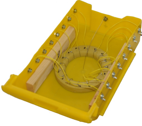
Fig. 9: Photograph of the phantom, built from a rubber gasket and stainless steel electrodes. The yellow dish is filled with a saline solution.
