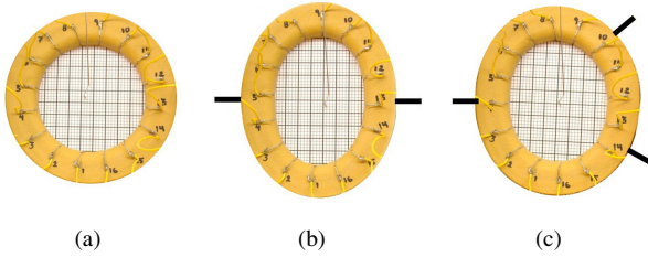
Fig. 10: Compressions: none (a), 2 points (b), 3 points (c)
