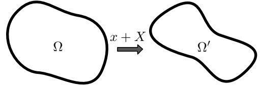
Fig. 4: A mapping of the domain \Omega to \Omega' by the vector field X
