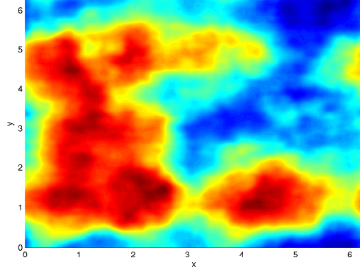
Fig. 1. Plot of two sample true solutions with 256 \times 256 modes at time T = 2 , (a) \gamma = 4 and (b) \gamma = 3 . Note the solution in (a) is smoother than the solution in (b) as the regularity of the noise decreases.
