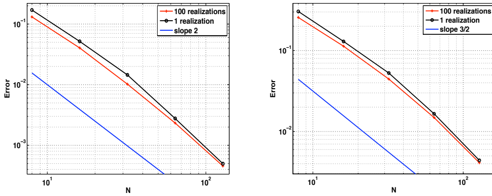
Fig. 2. Convergence in space for (a) \gamma = 4 and (b) \gamma = 3 . Plot is a log log plot of the error on [0, 2] , i.e. of \max_{t \in [0, 2]} \|u(t, \omega) - u^N(t, \omega)\|_H for the single realisation and of \max_{t \in [0, 2]} \left( \frac{1}{100} \sum_{i=1}^{100} \|u(t, \omega_i) - u^N(t, \omega_i)\|_H^2 \right)^{1/2} for the mean over 100 realisations, as the system size N is changed. Results are plotted for a single realisation and for the mean over 100 realisations. In (a) we see the predicted rate of N^{-2} and in (b) N^{-3/2} .
