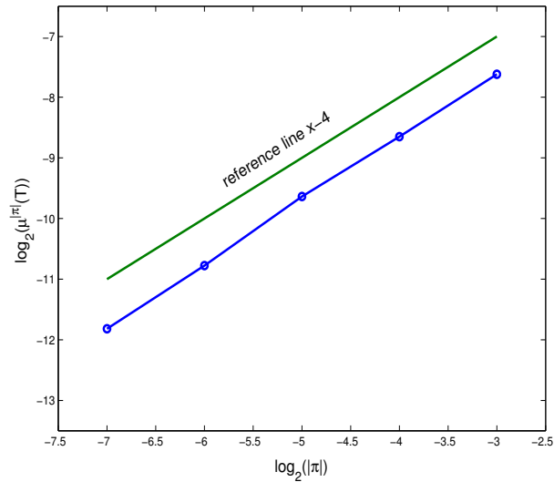
FIGURE 1. \log_2(\mu^{|\pi|}(T)) versus \log_2(|\pi|) for the solution of (??).
