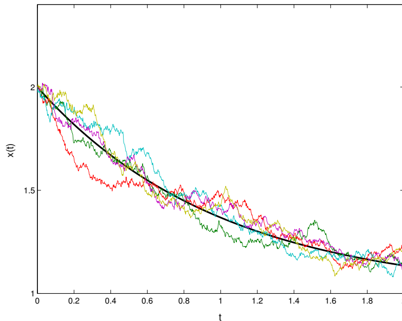
FIGURE 2. Trajectories of the solution of (?).
