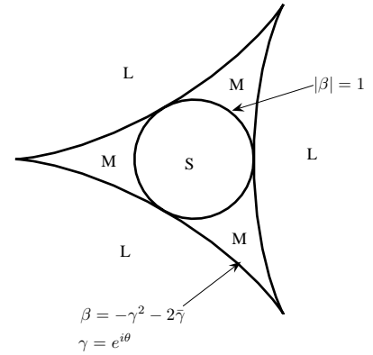
Figure 5: The relationship of lemon (L), monstar (M) and star (S) in the complex plane
