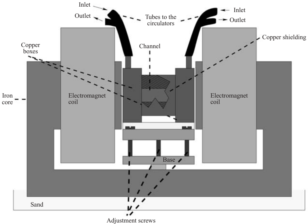
FIGURE 4. Experimental apparatus.
