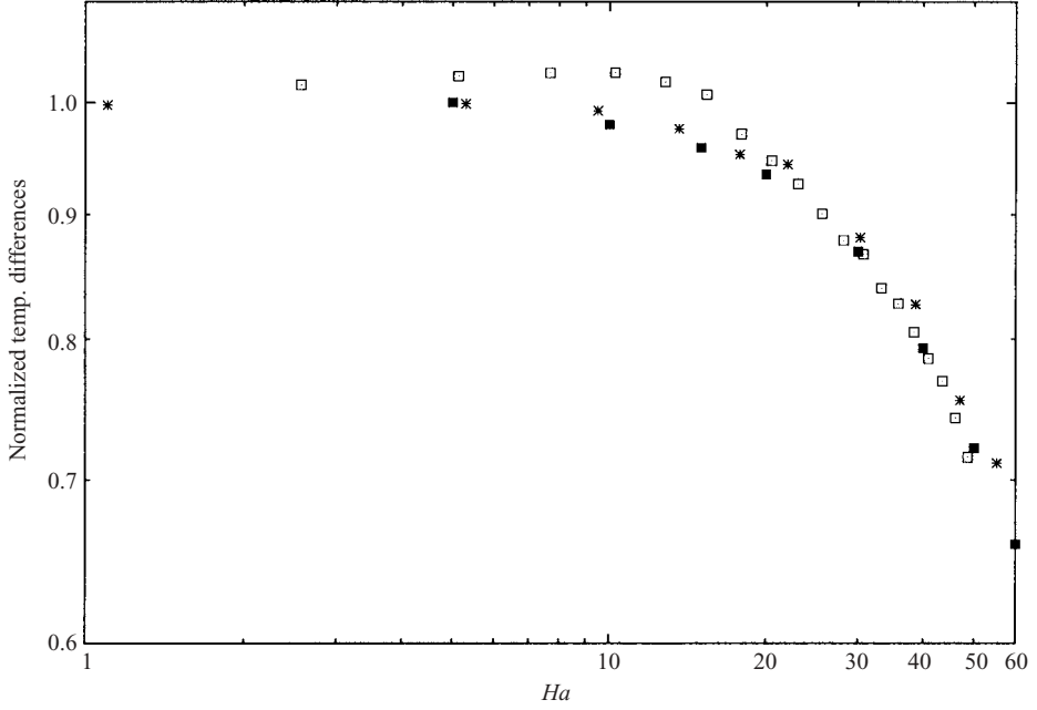
FIGURE 9. Comparison of the data of Juel et al. (1999) (■, numerical data; *, experimental data) to the experimental data of the present study (□). All data sets are normalized.
