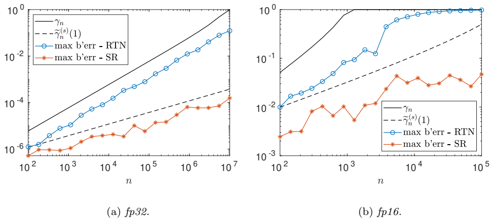
Fig. 5.1: Computed backward errors of inner products for random constant vectors in fp32 (a) and fp16 (b). For each value of n we perform the computation 10 times and plot the maximum backward error for round to nearest (RTN) and stochastic rounding (SR).
