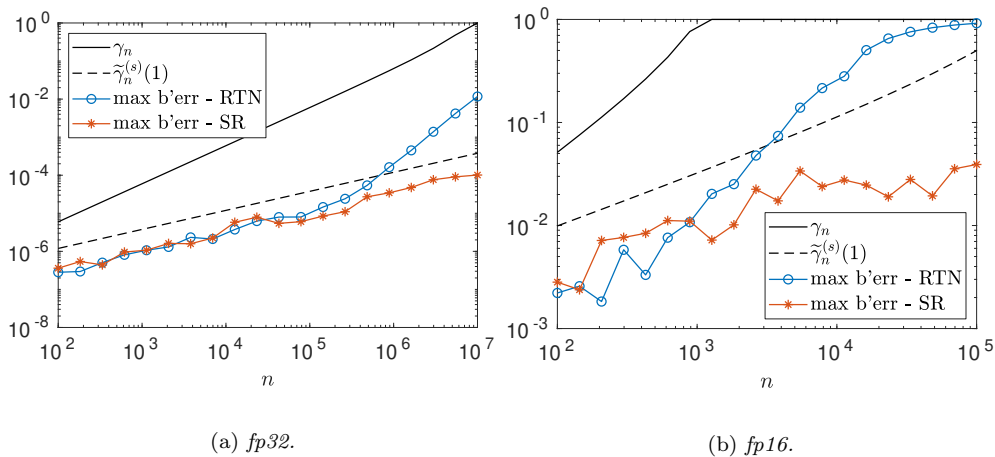
Fig. 5.2: Computed backward errors of inner products for data sampled from [0, 1] in fp32 (a) and fp16 (b). For each value of n we perform the computation 10 times and plot the maximum backward error for each rounding mode.
