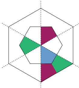
FIGURE 3. \Delta and the intersections of its translates with X^\vee .
