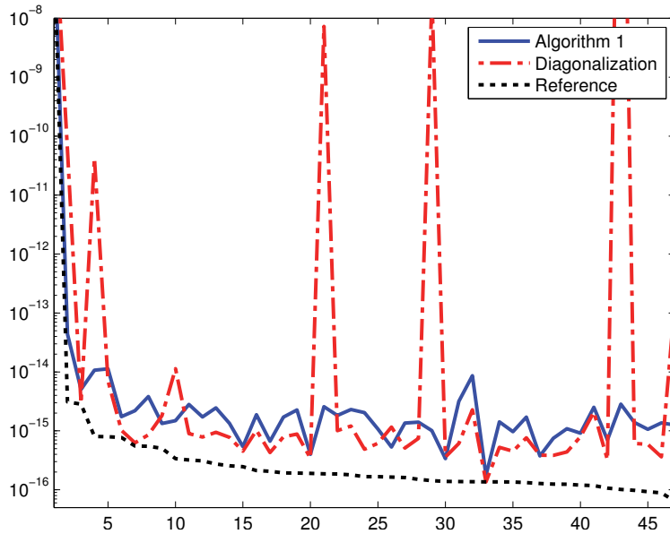
FIG. 5. Residuals in computing W_0(A) , where A \in \mathbb{C}^{n \times n} ranges over a set of 47 matrices chosen from the MATLAB gallery function. The results are ordered by nonincreasing residual of the reference solution.
