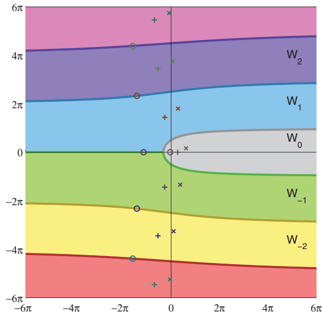
FIG. 1. The ranges of the branches of the Lambert W function and the values of W_k(1) (+), W_k(10 + 10i) ( \times ), and W_k(-0.1) (o). The colors of the curves that separate two adjacent regions denote the branches to which the curves belong. The corresponding plot for the logarithm consists of horizontal strips of height 2\pi with boundaries at odd multiples of \pi .
