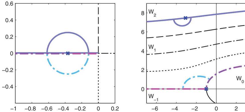
FIG. 2. The image through W_1(z) (right) of a region of the complex plane with a highlighted circle around the branch point -1/e (left). The image of the branch cut (-\infty, 0) when we approach it from above is the regular curve separating the range of W_1(z) from the range of W_2(z) ; while the image of the same half line when we approach it from below splits in two curves meeting at the point -1 : the left one separates the range of W_1(z) from that of W_{-1}(z) ; the right one separates the same range from that of W_0(z) . This illustrates why we treat in a different way the branch W_1(z) when we approach the negative real axis clockwise or counter-clockwise; we can loosely say that there is one branch cut from above and two from below. The colors have been used to show what the image of any (part of a) branch cut is.
