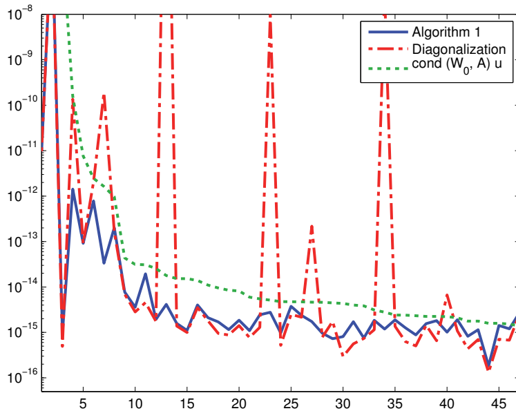
FIG. 6. Relative errors in computing W_0(A) , where A \in \mathbb{C}^{n \times n} ranges over 47 matrices chosen from the MATLAB gallery function. The results are ordered by nonincreasing value of \text{cond}(W_0, A)u .
