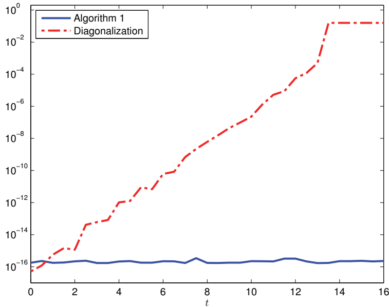
FIG. 4. Relative errors in computing W_{-1}(A) , with A of (5.1), with \varepsilon = 10^{-t} , for Algorithm 1 and the eigenvector approach.
