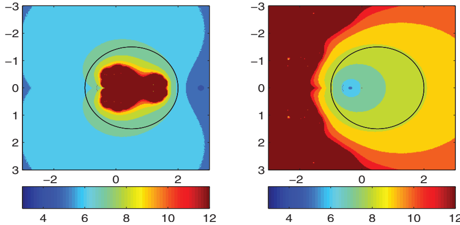
FIG. 3. Level curves revealing the convergence of Newton's method to W_0(z) with |\operatorname{Re} z| \leq 3 and |\operatorname{Im} z| \leq 3 by choosing z_0 = \varphi_0(z) (left) and z_0 = \psi_0(z) (right), together with the circle |z - 1/2| \leq 3/2 . Dark blue means less than four iterations for convergence, while dark red means more than 11 or lack of convergence.
