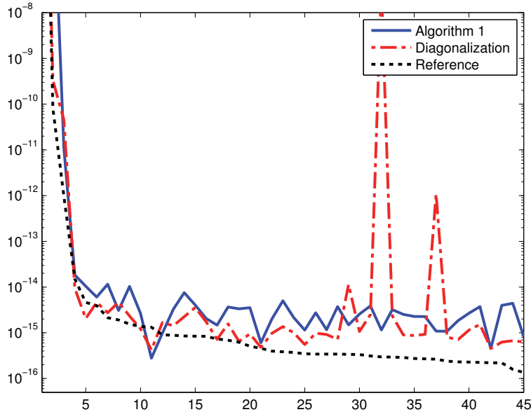
FIG. 7. Residuals in computing W_{-1}(A) , where A \in \mathbb{C}^{n \times n} varies over 45 matrices chosen from the MATLAB gallery function. The results are ordered by nonincreasing residual of the reference solution.
