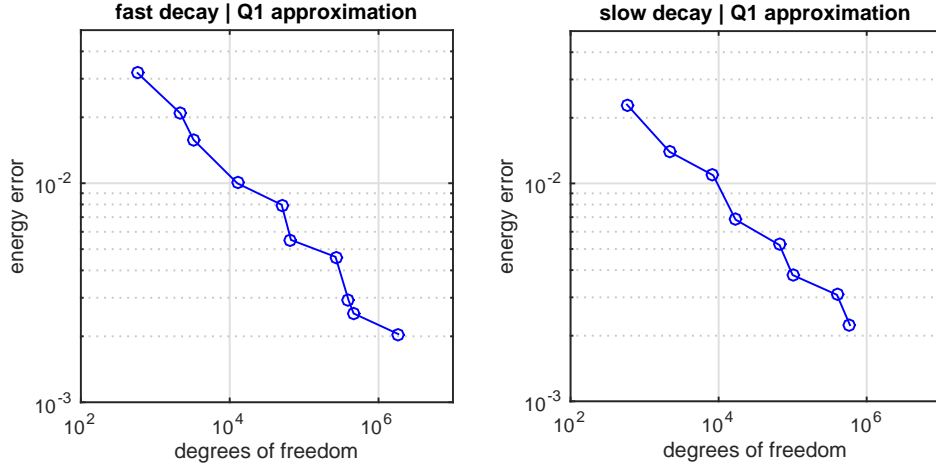
FIG. 6.1. Error estimates at each step of the adaptive algorithm using Q_1 spatial approximation, with fast ( \bar{\sigma} = 4 ) and slow ( \bar{\sigma} = 2 ) decay of the amplitude coefficients.
