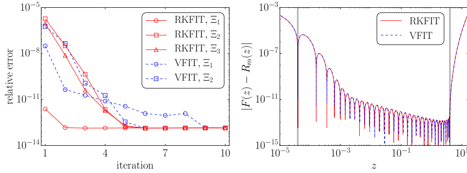
Fig. 5.2: Least-squares approximation of the function F(z) = z^{1/2} using RKFIT and the vector fitting code VFIT. Left: This plot shows the relative approximation error \|F(A)\mathbf{v} - R_m(A)\mathbf{v}\|_2 / \|F(A)\mathbf{v}\|_2 after each iteration of RKFIT (solid red) and VFIT (dashed blue). The convergence curves for each method correspond to different choices for the initial poles \Xi_1 (circles), \Xi_2 (squares), and \Xi_3 (triangles), respectively. Right: This is the plot of |F(z) - R_m(z)| over an interval on the positive real axis obtained after 10 iterations of RKFIT and VFIT with initial poles \Xi_1 . The vertical lines indicate the spectral interval of A .
