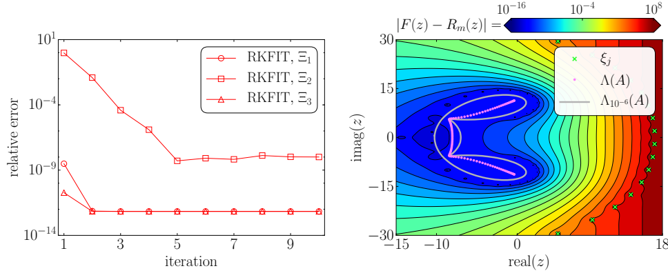
Fig. 5.3: Least-squares approximation of the function F(z) = \exp(z) using RKFIT. Left: This plot shows the relative approximation error \|F(A)\mathbf{v} - R_m(A)\mathbf{v}\|_2 / \|F(A)\mathbf{v}\|_2 after each iteration of RKFIT (solid red) for different choices of initial poles \Xi_1 , \Xi_2 , and \Xi_3 , respectively. Right: A plot of |F(z) - R_m(z)| over a region in the complex plane together with the poles of R_m (green crosses), where R_m is the rational least squares approximant obtained after 10 iterations of RKFIT with initial poles \Xi_1 . The eigenvalues of the Grcar matrix and its 10^{-6} -pseudospectrum are also shown.
