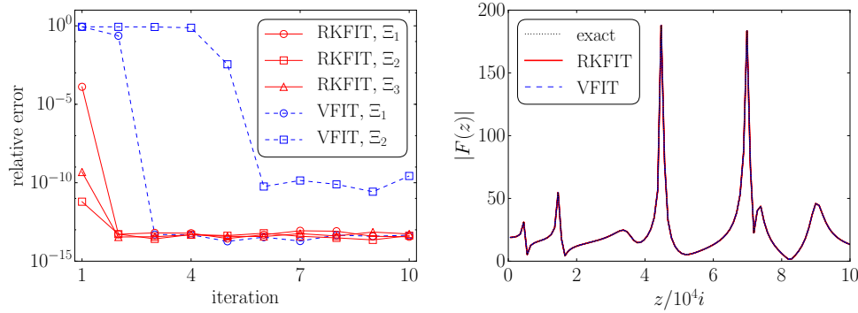
Fig. 5.1: Least-squares approximation of a rational function F(z) of type (19, 18) using RKFIT and the vector fitting code VFIT. Left: Relative error \|F(A)\mathbf{v} - R_m(A)\mathbf{v}\|_2 / \|F(A)\mathbf{v}\|_2 after each iteration of RKFIT (solid red) and VFIT (dashed blue). The two convergence curves for each method correspond to different choices for the initial poles \Xi_1 (circles), \Xi_2 (squares), and \Xi_3 (triangles), respectively. Right: Plot of |F(z)| over an interval on the imaginary axis overlaid with the approximants |R_m(z)| obtained after 10 iterations of RKFIT and VFIT with initial poles \Xi_1 (the curves are visually indistinguishable).
