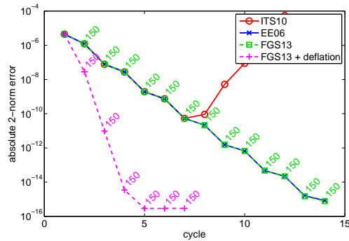
FIG. 5.4. Approximating (e^{-s\sqrt{A}} - I)A^{-1}\mathbf{b} : Convergence history (left) and running times (right) for the different restarting procedures. The restart length is m = 50 in all cases, and in the variant with deflation a number of d = 5 Ritz vectors was used.
