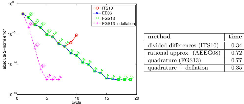
FIG. 5.1. Approximating A^{-1/2}\mathbf{b} : Convergence history (left) and running times (right) for the different restarting algorithms. The numbers next to the curves for the new quadrature-based methods indicate the number of quadrature nodes used for evaluating the error function in the corresponding restart cycle. The restart length is m = 50 in all cases, and in the variant with deflation a number of d = 5 Ritz vectors was used.
