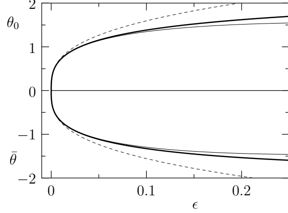
Figure 5: Plot of \bar{\theta} and \theta_0 versus \epsilon for \varrho = 1 . The thick solid line represents the numerical solution. The one-term approximation (dashed line) agrees with the numerical solution only for very small values of \epsilon . The two-term asymptotic expression (solid thin line) gives a much better agreement on a wider range of \epsilon .
