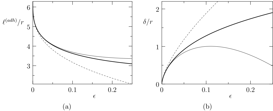
Figure 6: Plot of (a) the adherence length, \ell^{(adh)}/r , and (b) the blister height, \delta/r , as functions of \epsilon , when \varrho = 1 . The solid thick lines are the numerical solutions, the dashed lines represent the one-term approximation while the solid thin lines show the two-term approximation. This latter approximation seems to describe the adherence length reasonably well, but it does not fully capture the behaviour of the blister height.
