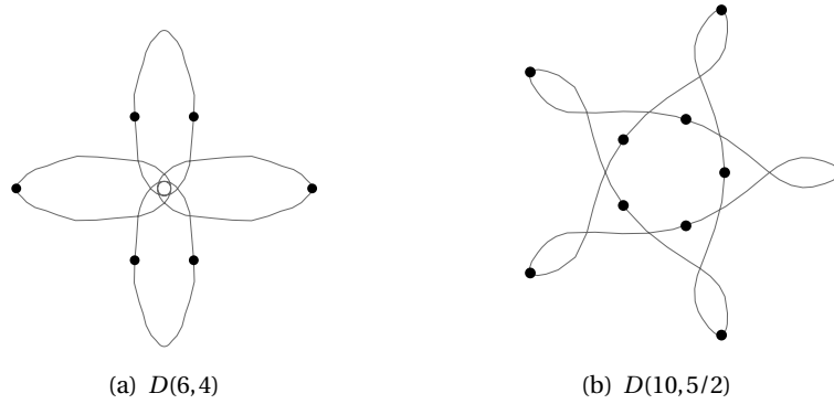
FIGURE 2.3: Two examples of choreographies with nontrivial core: in the first the order of the core is c = 2 and in the second c = 5 .
