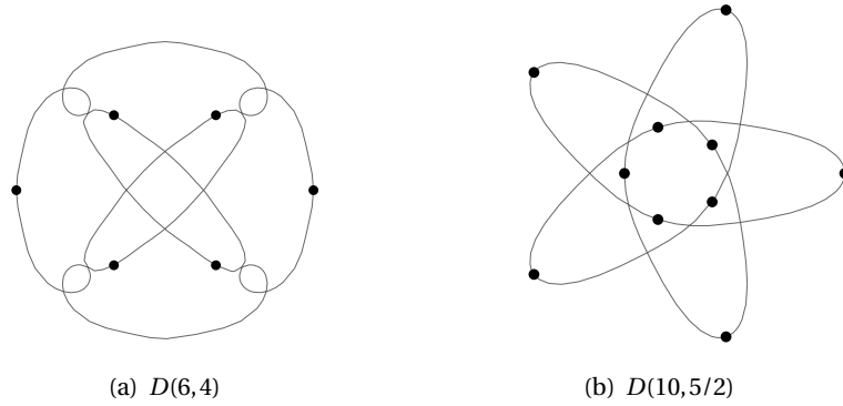
FIGURE 5.3: Two examples illustrating different connected components of each symmetry type compared with those in Figure 2.3. Many examples of 5-body choreographies with a single time-reversing reflectional symmetry—so type D(5, 1) —in different connected components have been found (numerically) by Simó [33, Figure 3].
