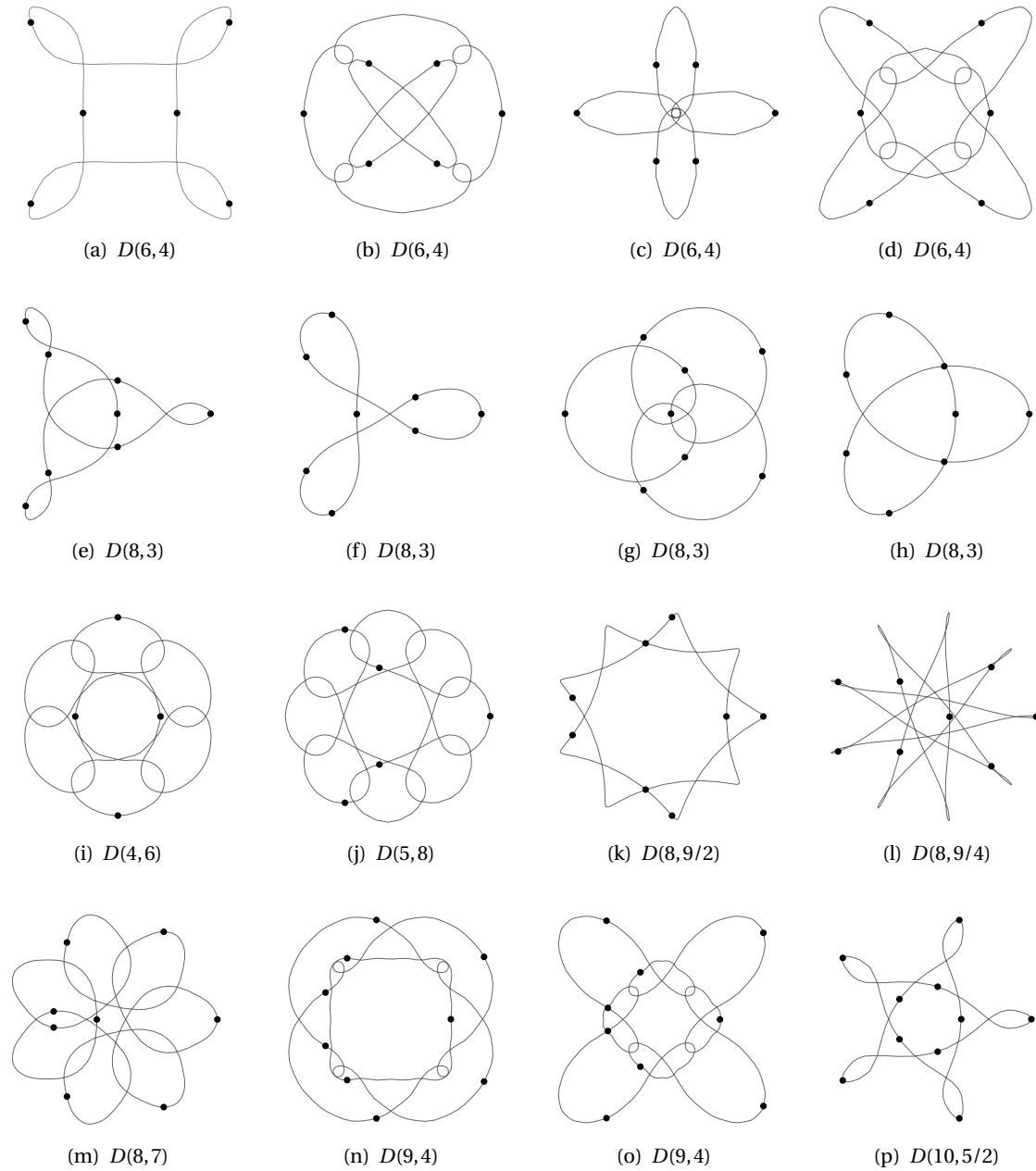
FIGURE 1.2: A selection of choreographies with their symmetry group. See Remark 1.6. These are all from the regular families of symmetry groups; for some examples illustrating the exceptional symmetry groups see Fig. 2.4. Where the same label appears for more than one figure, they correspond to different connected components of the corresponding \text{Fix}(G, \Lambda X^{(m)}) . Animations can be seen at [25].
