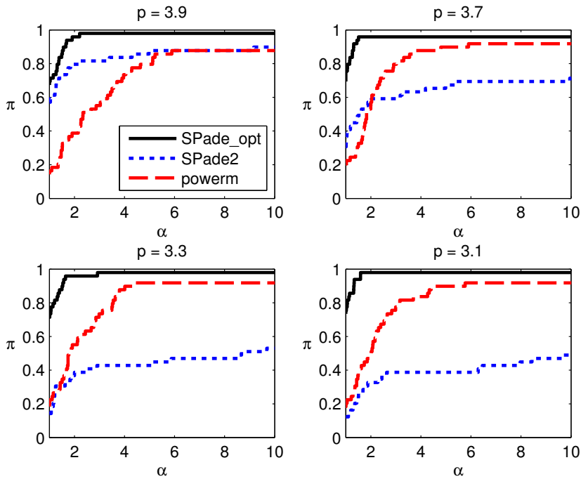
FIG. 9.8. Experiment 6: performance profile of relative errors. The legend for first plot applies to all four plots. \text{SPade2} uses p_2 in (6.1b) and \text{SPade\_opt} uses the choice defined in Section 6.
