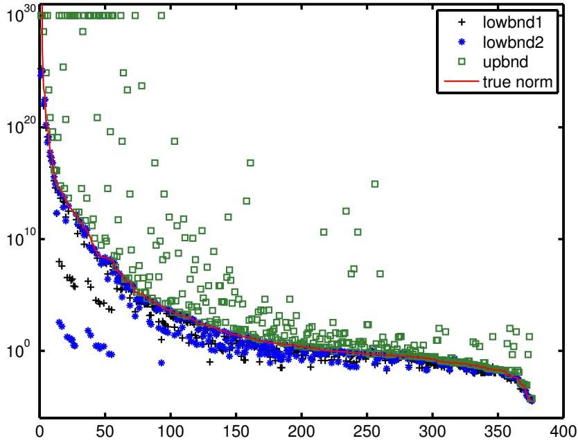
FIG. 9.7. Experiment 5: the lower bounds \text{lowbnd1} in (2.7) and \text{lowbnd2} in (2.8), the upper bound \text{upbnd} in (2.8), and the true norm \|L_{x^p}(A)\|_F , for the matrices in Experiment 3.
