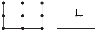
Fig. 1. Q_2\text{-}P_{-1} element ( \bullet velocity node; \circ pressure; \dagger pressure derivative).
