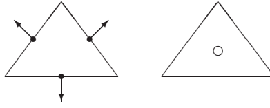
Fig. 3. RT_0 element (• normal velocity component; ◦ pressure).
